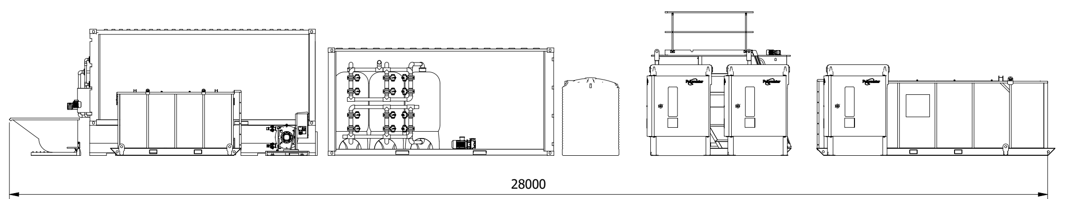
ELEVATION VIEW
